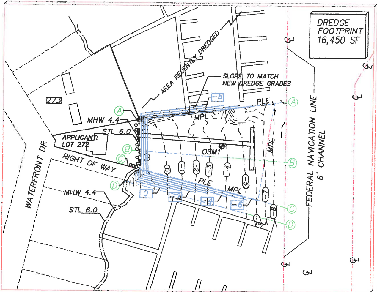
PLAN VIEW 1"=80'
