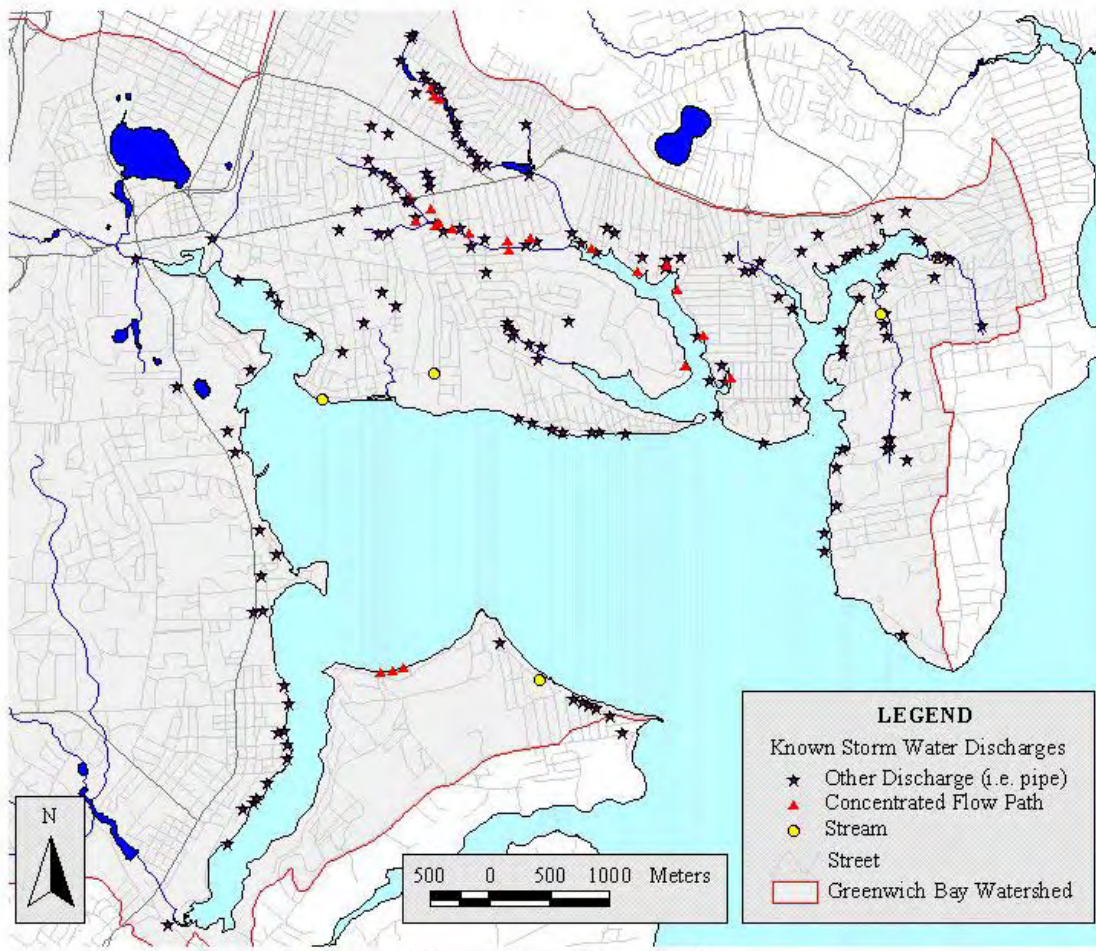
Figure 11. Approximate locations of stormwater outfalls
