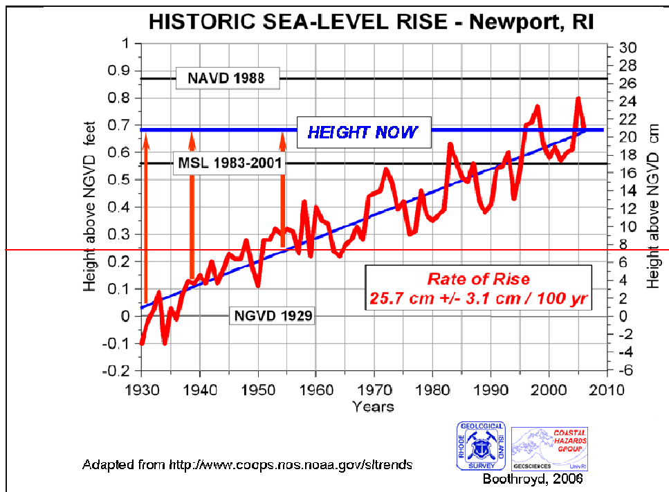
Figure 1. Historic Sea level Rise in Newport, RI shows an increase of approximately 0.64 feet between 1930 and 2006
