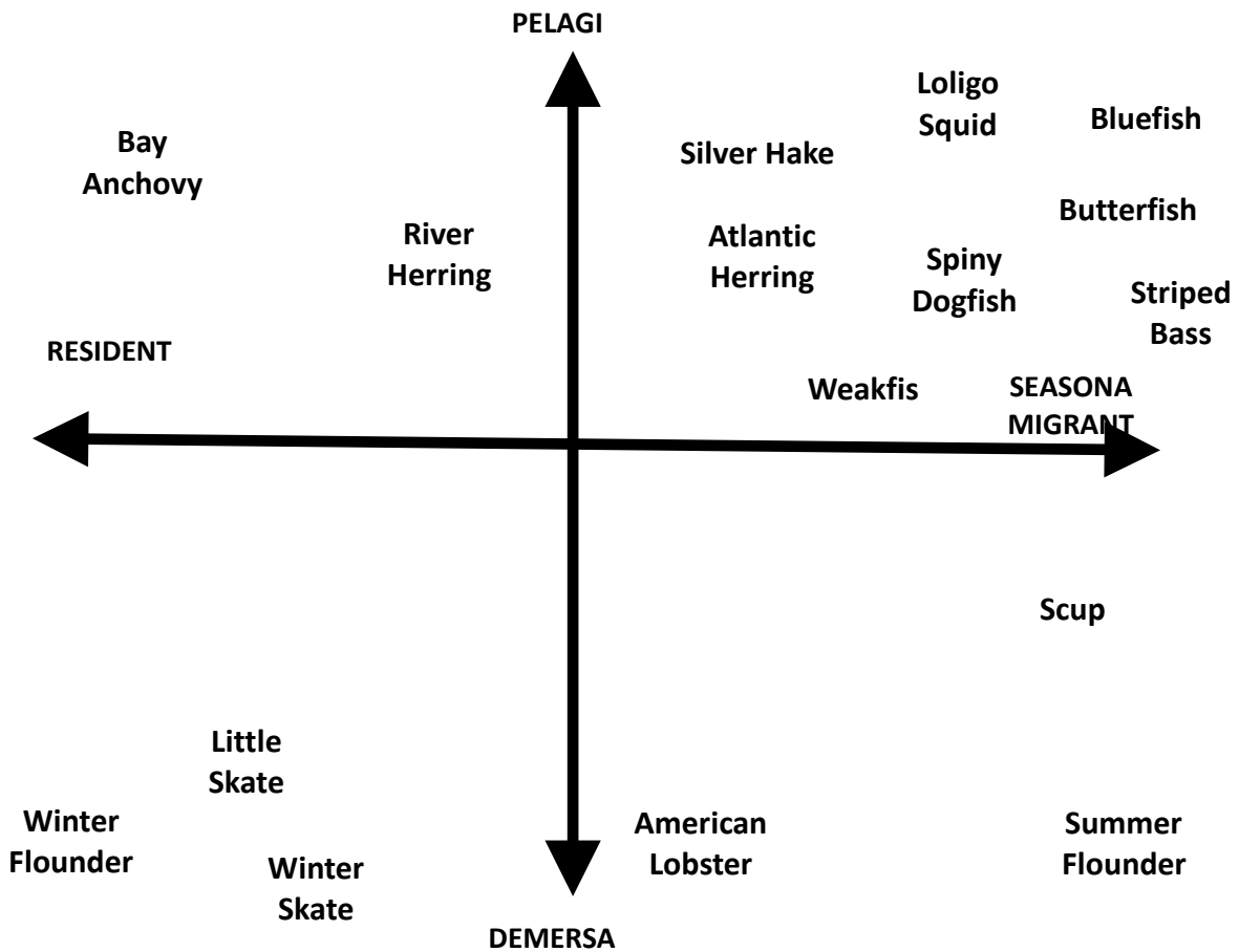
Figure 2.27. Seasonal composition of major fish and invertebrate species in the Ocean SAMP area (from Brown 2009).
