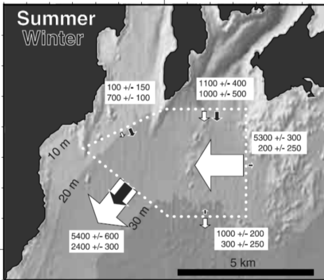
Figure 2.20. Seasonal, tidally averaged volume transport between Narragansett Bay and Rhode Island Sound (from Kincaid et al. 2003). White arrows are for summer flows and black for winter; size of arrow is relative to volume of flow; units are m^3 \cdot sec^{-1} .
