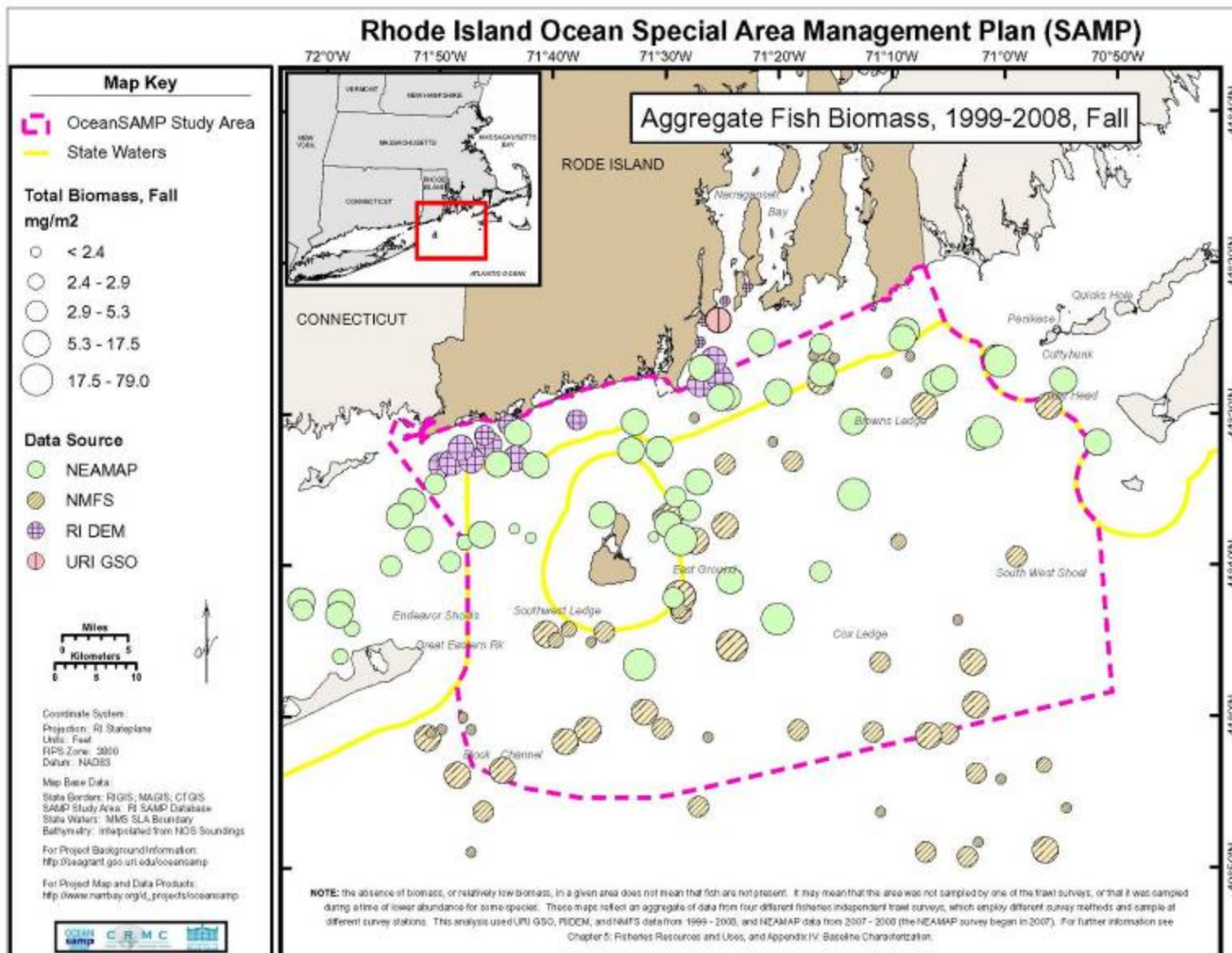
Figure 5.4. Aggregate fish biomass, 1999-2008, fall.
