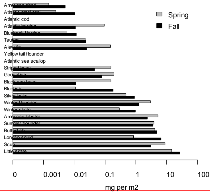
Figure 5.7. GSO trawl survey biomass per area by species. (Bohabor et al. 2010)
