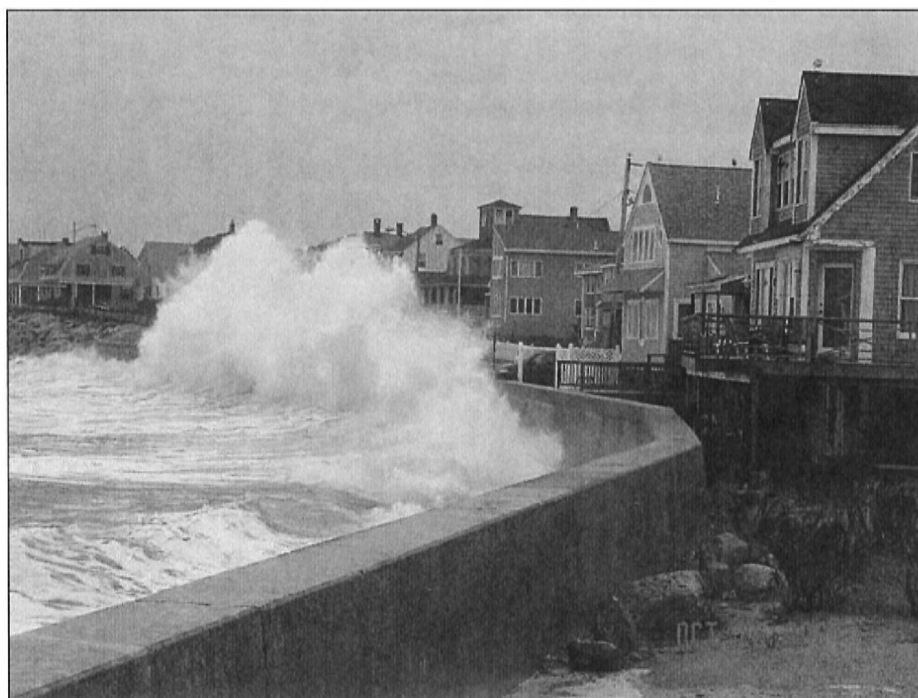
Figure 1. Vertical concrete seawall with toe stones protecting waterfront buildings from the direct impact of storm waves along the South Shore of Massachusetts.
