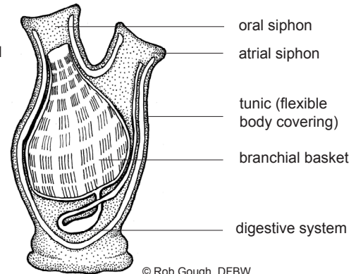
Anatomy of an individual tunicate
