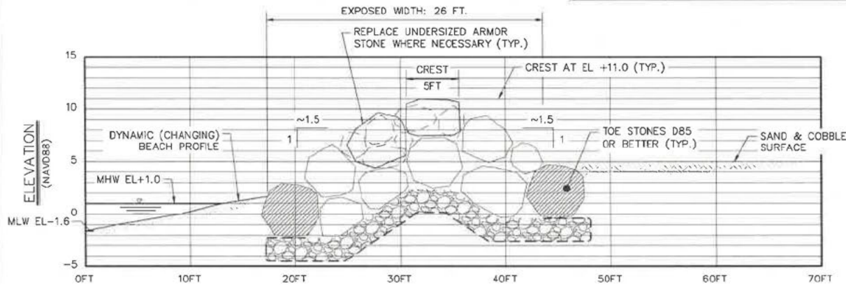
SECTION B-B PROPOSED
