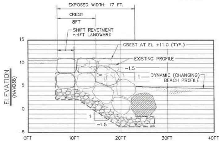
SECTION D-D PROPOSED
