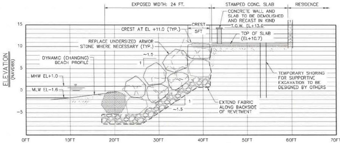
SECTION C-C PROPOSED
