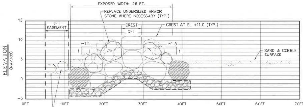
SECTION A-A PROPOSED
