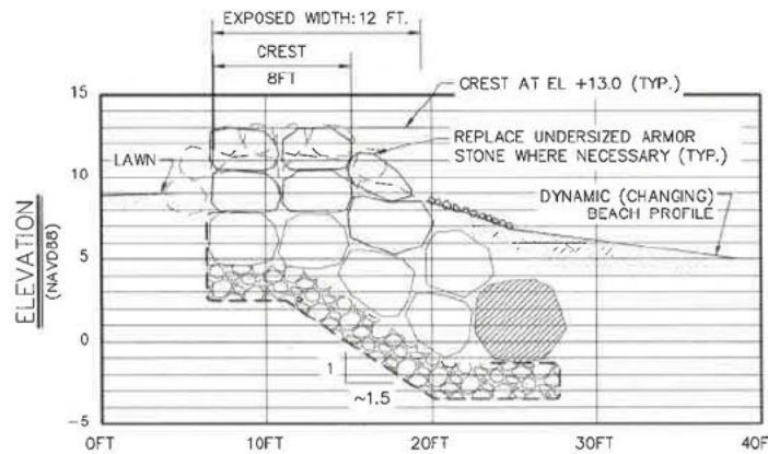
SECTION E-E PROPOSED
