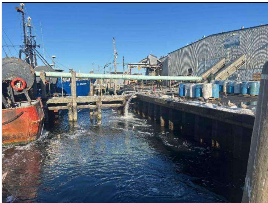
Photo No. 3.: View of the landside connection to the bulkhead of Pier 'JJ' looking north. (Photo 12/18/2025)
