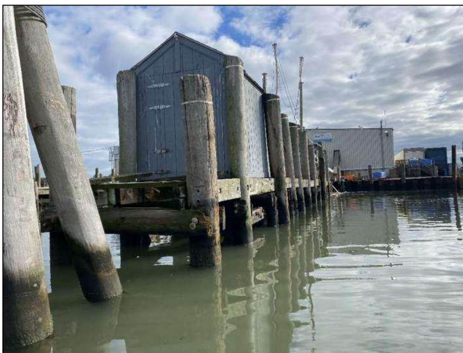
Photo No. 2.: View of Pier 'JJ' looking toward the bulkhead.
