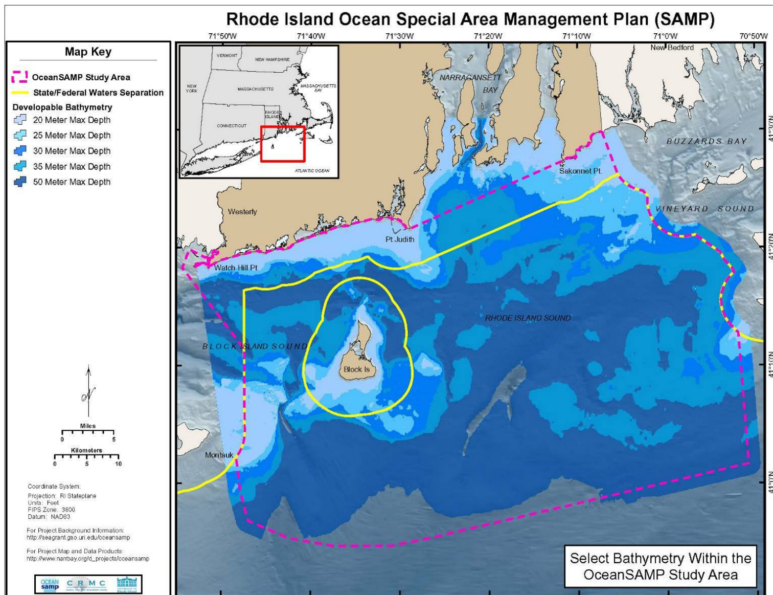
Figure 8.23. Ocean SAMP Area Bathymetry.
